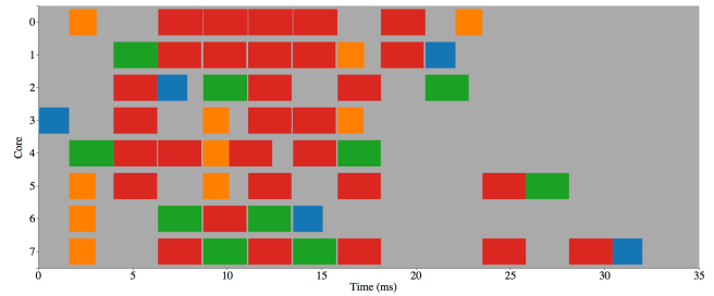
Figure 2: This is an example of a trace from the same numerical linear algebra application in Figure 1. The tasks are colored to match the task classes in Figure 1.
