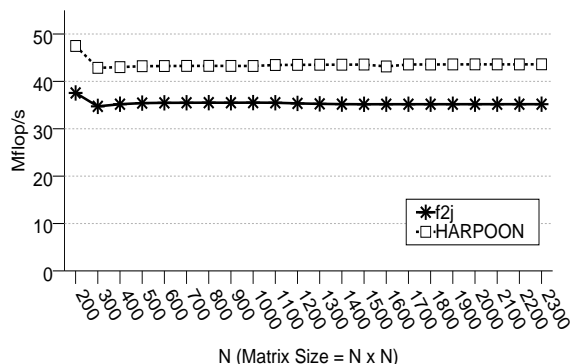
Figure 3: Comparison of f2j-generated DGEMM with Object-oriented Version
