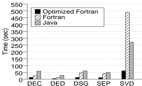
Figure 2: Elapsed Time Executing Various LAPACK Test Routines
